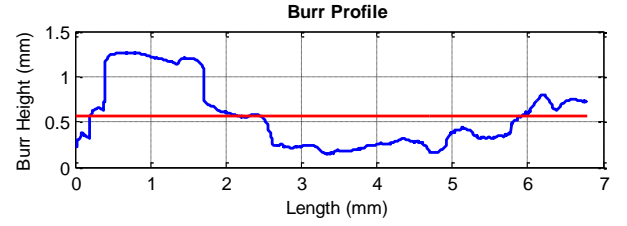
Figure 4. Measured burr profile [7]
