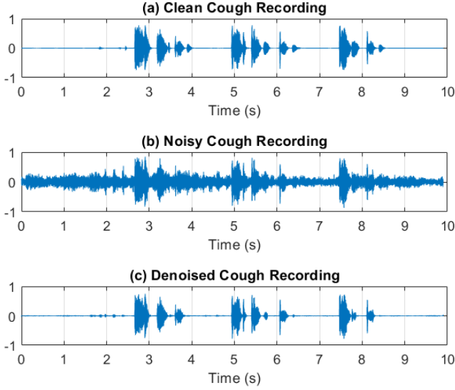
Fig. 7. Waveform of (a) clean cough recording, (b) noisy cough recording, and (c) denoised using FNN cough recording.
